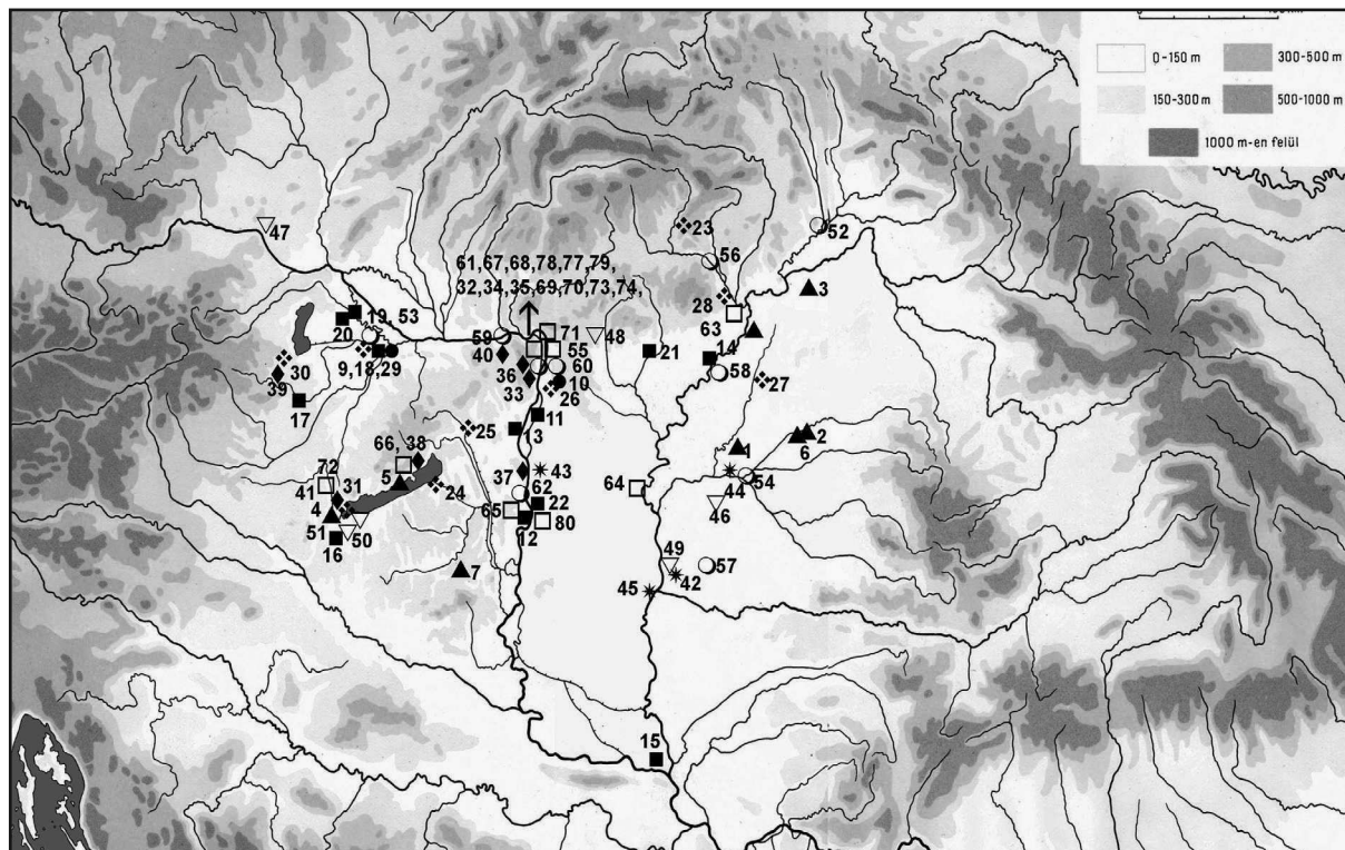
Fig 1. Broomcorn millet sites in the Carpathian Basin
