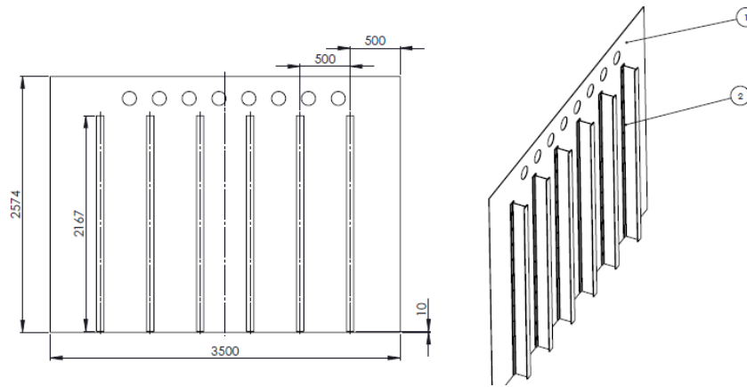
Fig. 2. Back part of the water chamber
