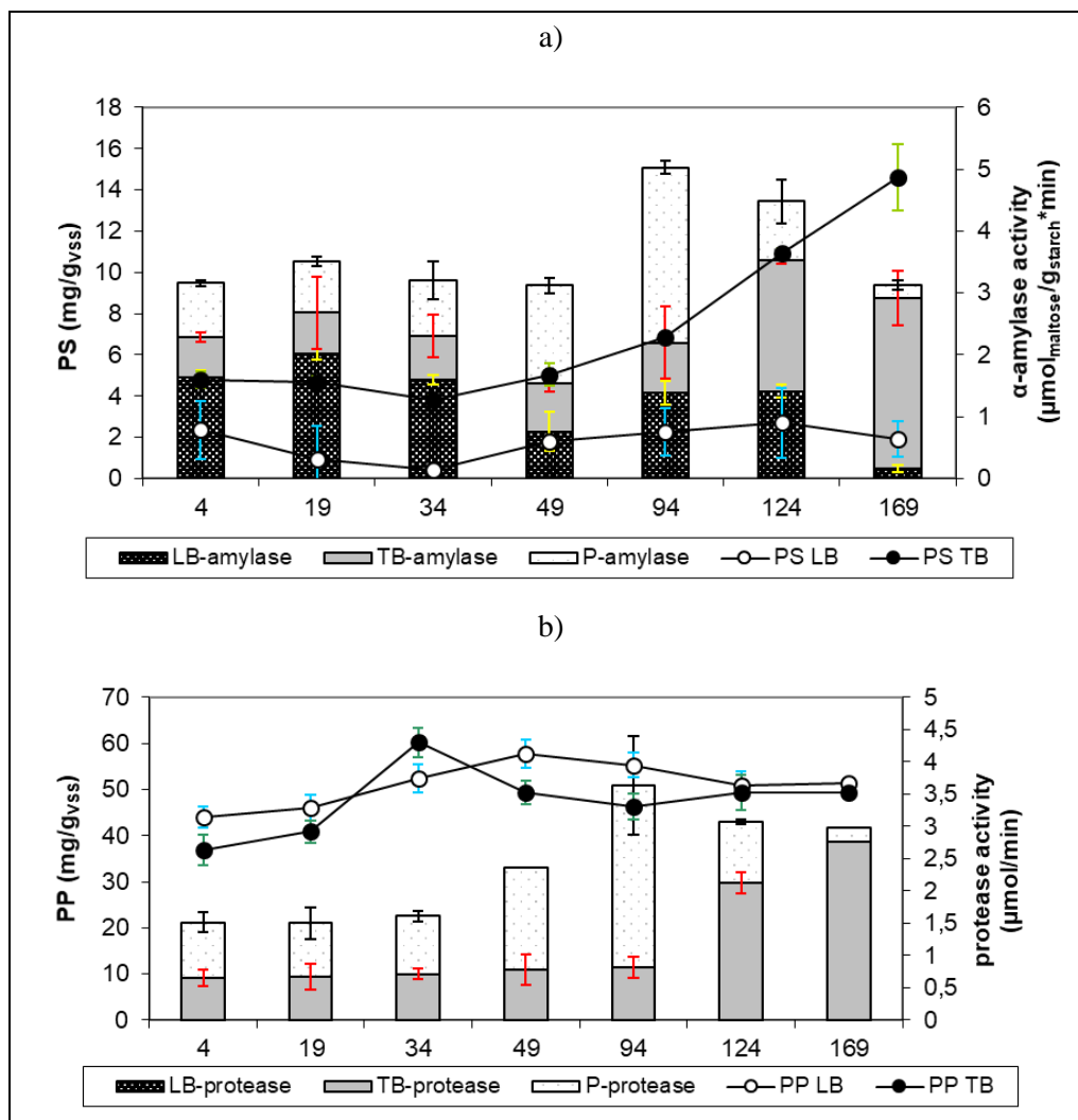
Figure 3. Dynamics of changes in amylase and protease activity during a single reactor cycle with granular sludge (30 th day of the granulation). Explanations: PP – polypeptides, LB – loosely-bound, PS – polysaccharides, TB – tightly-bound, P – pellets. *vertical bars – standard deviation
