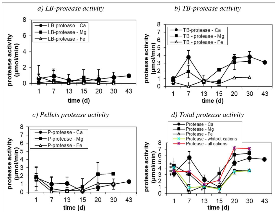
Figure 1. The influence of \text{Ca}^{2+} , \text{Mg}^{2+} and \text{Fe}^{3+} on the change of protease activity a) in LB-EPS-fraction (loosely bound EPS), b) in TB-EPS-fraction (tightly bound EPS), c) in P-EPS (EPS in pellets) and on the change of the total protease activity (d) (vertical bars – standard deviation, * - no statistical significance, p < 0.05 )
