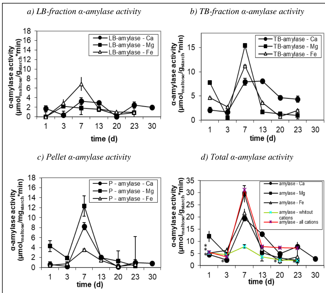
Figure 2. The influence of \text{Ca}^{2+} , \text{Mg}^{2+} and \text{Fe}^{3+} on the change of amylase activity a) in LB-EPS fraction, b) in TB-EPS fraction, c) in P-EPS fraction (pellets) and on the change of the total amylase activity (d) (vertical bars – standard deviation, * - no statistical significance, p < 0.05 )
