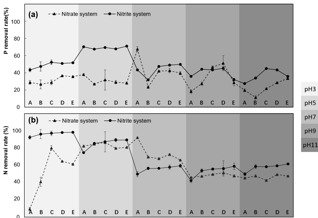
Figure 6. Removal rate of phosphate (a) nitrogen (b) during the cycle. From A to E represent the concentration of nitrate ( 10 \text{ mg L}^{-1} , 20 \text{ mg L}^{-1} , 30 \text{ mg L}^{-1} , 40 \text{ mg L}^{-1} and 50 \text{ mg L}^{-1} , respectively) and nitrite ( 1 \text{ mg L}^{-1} , 2 \text{ mg L}^{-1} , 3 \text{ mg L}^{-1} , 4 \text{ mg L}^{-1} and 5 \text{ mg L}^{-1} , respectively)
