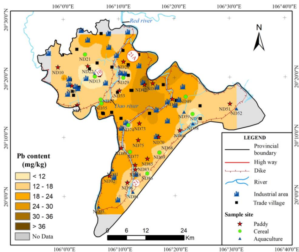
Figure 8. Distribution of Pb in the topsoil of the agricultural soil in Nam Dinh province
