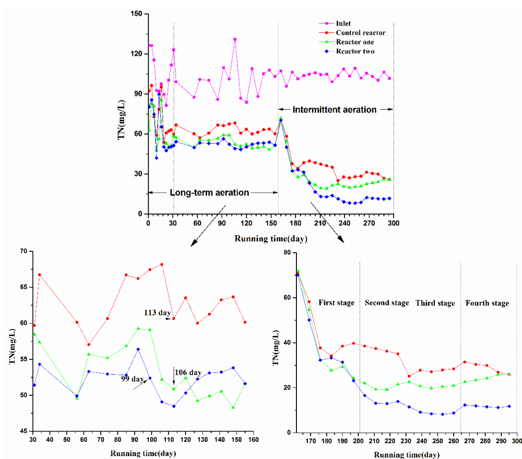
Figure 11. Changes of TN concentration in the influent and effluent
