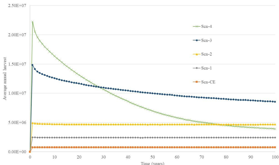
Figure 3. Average weight of female SMA harvest as a function of time for each harvest scenario (Scn-CE, Scn-1, Scn-2, Scn-3 and Scn-4)
