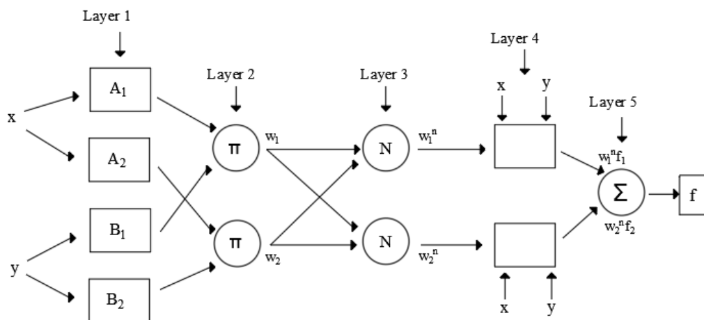
Figure 3. ANFIS architecture
