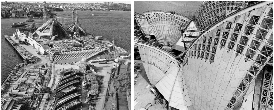
Figure 10. The construction of the gigantic roofs with on-site prefabrication
