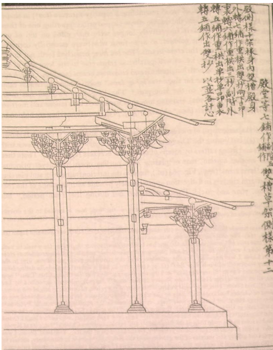
Figure 3. A page from the more than 900 year old Chinese Yingzao fashi
