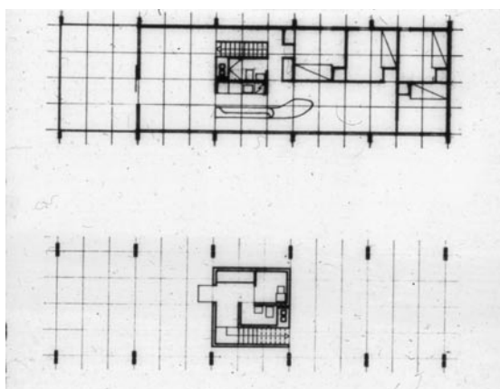
Figure 5. The Utzons' first custom designed family house
