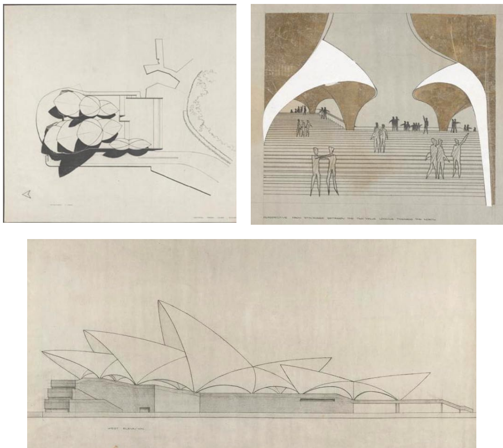
Figure 7. A few sheets from Utzon's entry
