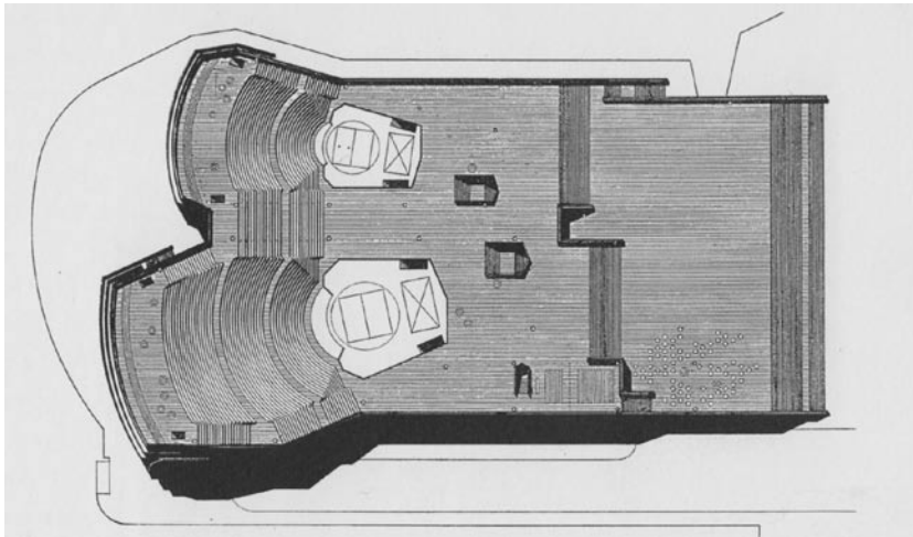
Figure 8. The tectonic base: the vast stepped 'solid' podium
