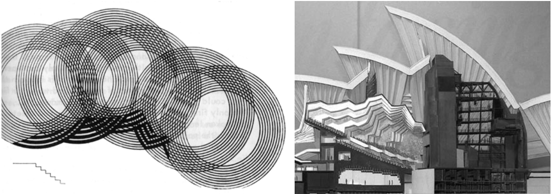
Figure 11. Utzon's proposal for the load bearing acoustic ceiling by undulating ply-wood beams using cylinder geometry
