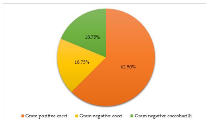
Figure 5. Total number of gram positive and gram negative bacteria in all four laboratories
