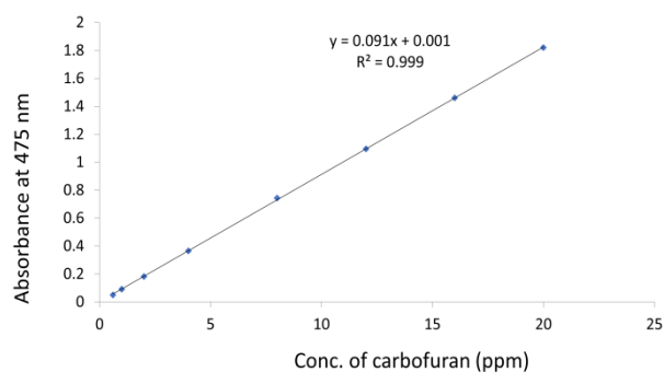
Figure 1. Standard calibration curve of carbofuran.
