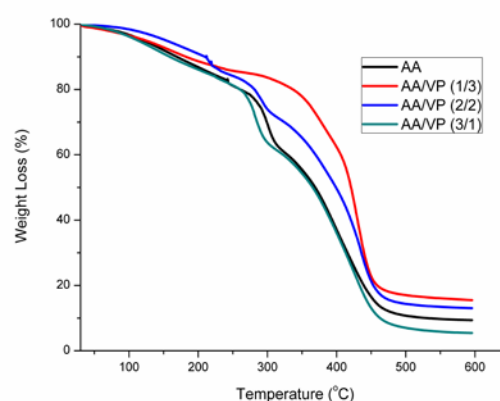
Figure 3. TGA curve of homo-polymeric AA and hetero-polymeric AA/VP in the ratio of 1:3, 2:2 and 3:1 hydrogels.
