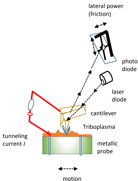
Figure 3. Tandem Nanoscope.
