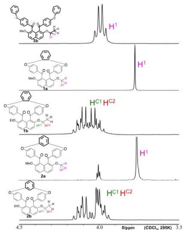
Figure 5. ^1\text{H} NMR study of compounds 3b , 1a , 1b , 2a , and 2b in \text{CDCl}_3 ( \delta 3.5–4.5 ppm).
