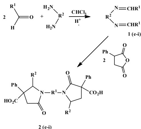
Scheme 2. Synthesis of ( E,Z )-bis \gamma -lactams.
