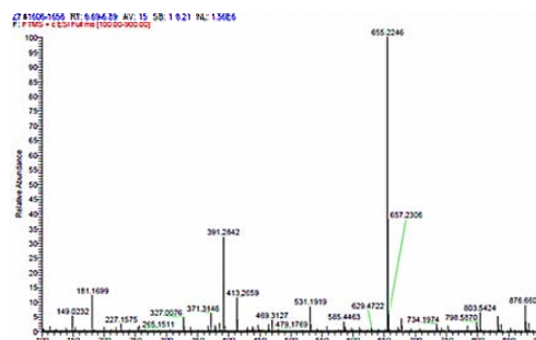
Figure 8. Mass spectrum of ( 2h ).
