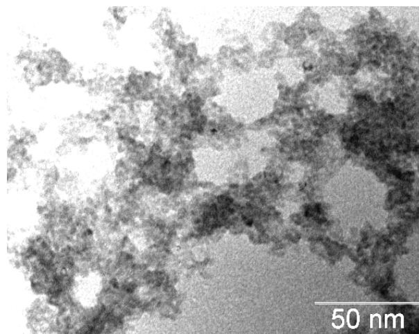
Figure 3. TEM image of the as synthesized zinc oxide nanoparticles
