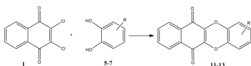
Scheme 2. Formation of benzodioxins from DCNQ 1 and catechols 5-7 .
