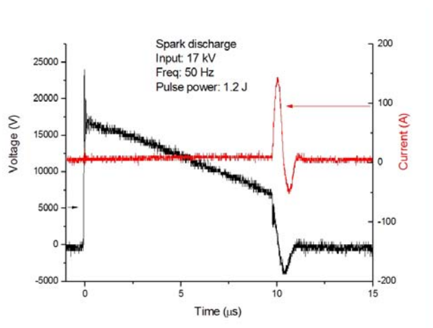
Figure 2. Typical voltage and current pulse of the spark electrohydraulic discharge
