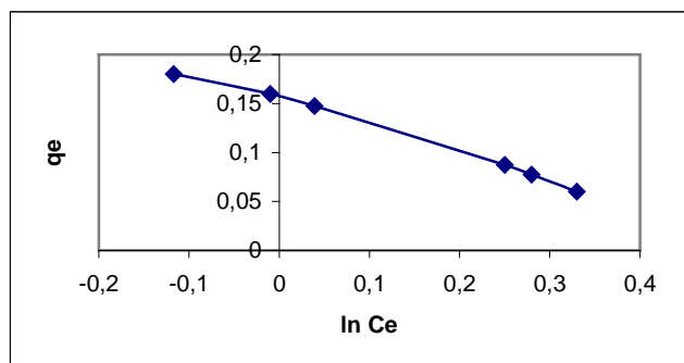
Figure 6. Temkin isotherm at 25 °C
