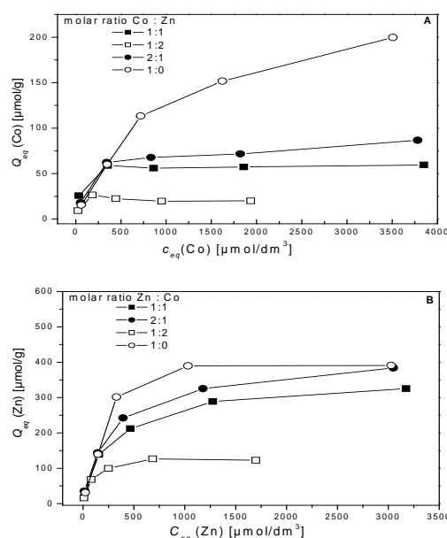
Figure 1. Cobalt (A) and zinc (B) sorption from binary system Co-Zn at variable initial molar [Co]: [Zn] ratios by dried activated sludge (2.5 g/dm 3 , d.w.) at 22°C and pH 6.0.
