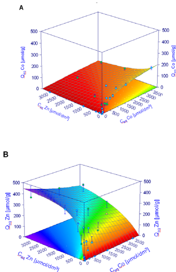
Fig. 3. 3-D sorption isotherm surfaces of \text{Co}^{2+} - \text{Zn}^{2+} binary system: (A) \text{Co}^{2+} sorption ( \mu\text{mol g}^{-1} ); (B) \text{Zn}^{2+} sorption ( \mu\text{mol g}^{-1} ). The sorption surfaces are predicted by the competitive Langmuir model (Eqs. 2 and 3) and the points present experimental data obtained at pH 6 and 22 °C. Error-bars represent 90% confidence interval.
